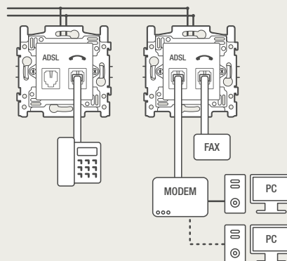
1 x TEL + 1 x FAX + 1 x ADSL
