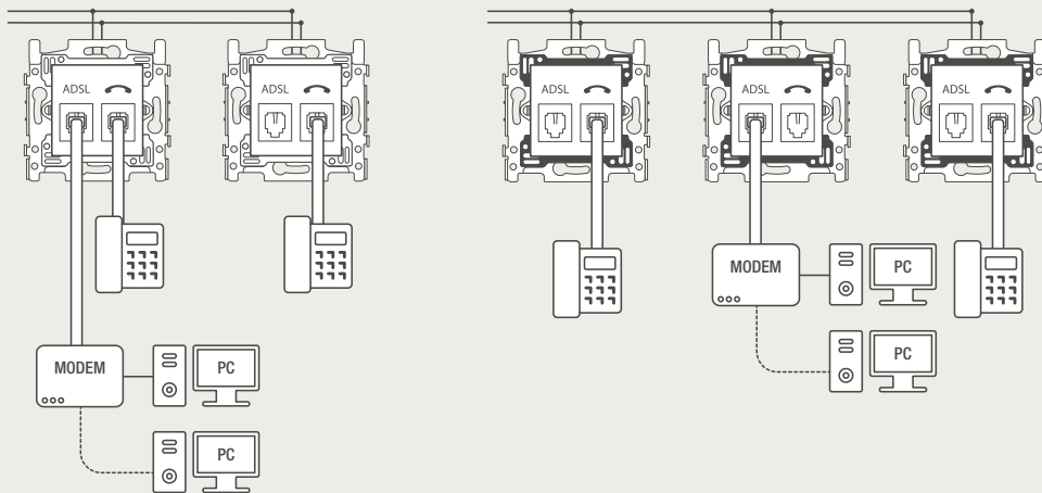
2 x TEL + 1 x ADSL
